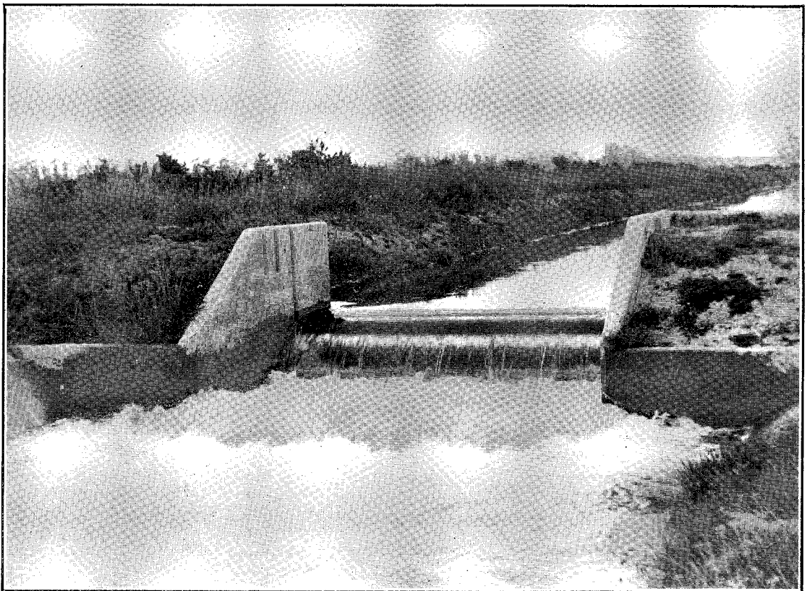
WATER-DROP IN OPERATION; CAPACITY, 180 CUBIC FEET PER SECOND. LEVELS IRRIGATION SCHEME.
