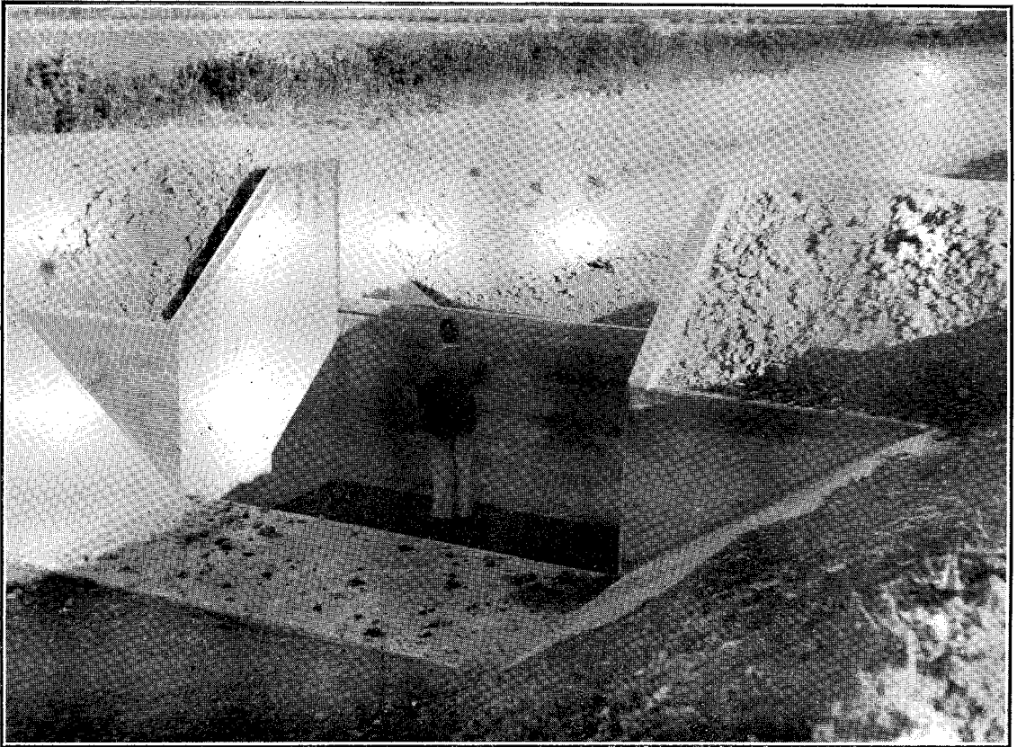
WATER-DROP COMPLETED; CAPACITY, 180 CUBIC FEET OF WATER PER SECOND.
