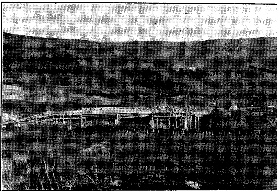
KAI IWI OVERBRIDGE, IN COURSE OF CONSTRUCTION, ELIMINATING LEVEL CROSSING SHOWN IN TOP VIEW.
