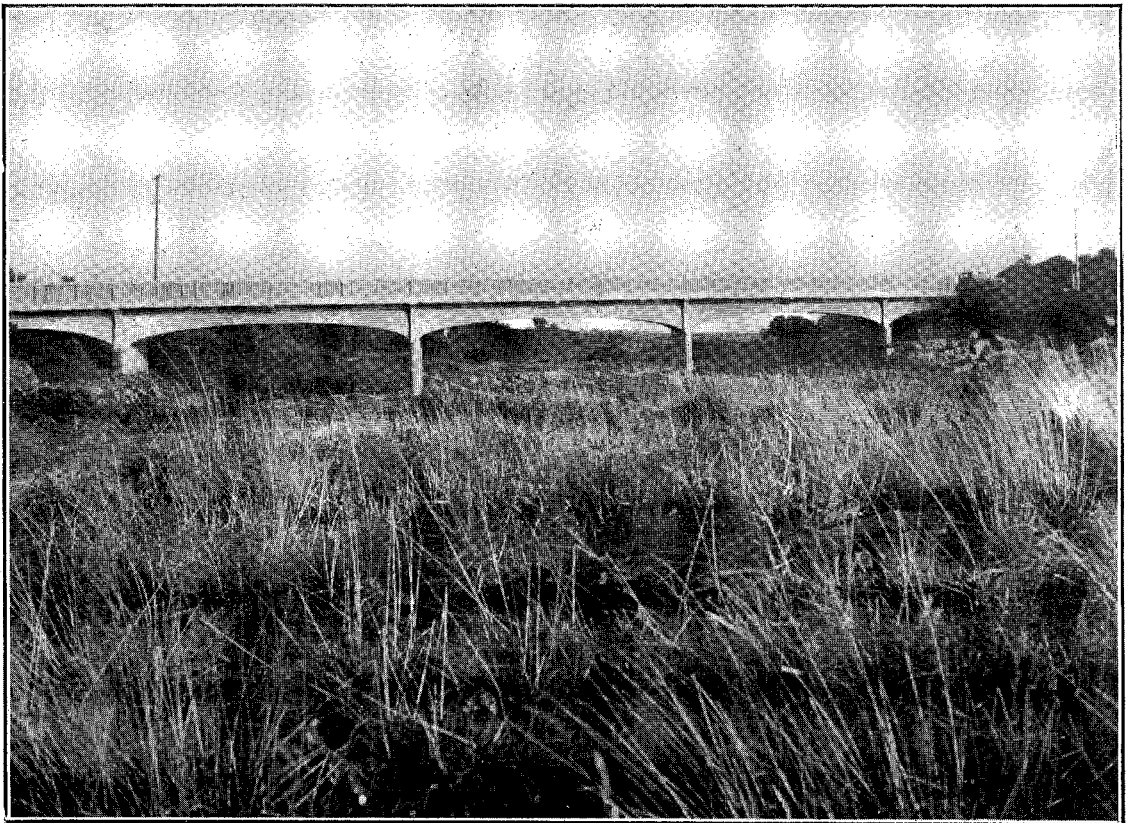
PUNEHU BRIDGE. ONE 65 FT., TWO 57 FT., AND TWO 20 FT. SPANS; 20 FT. ROADWAY. EITHAM-OPUNAKE MAIN HIGHWAY.
