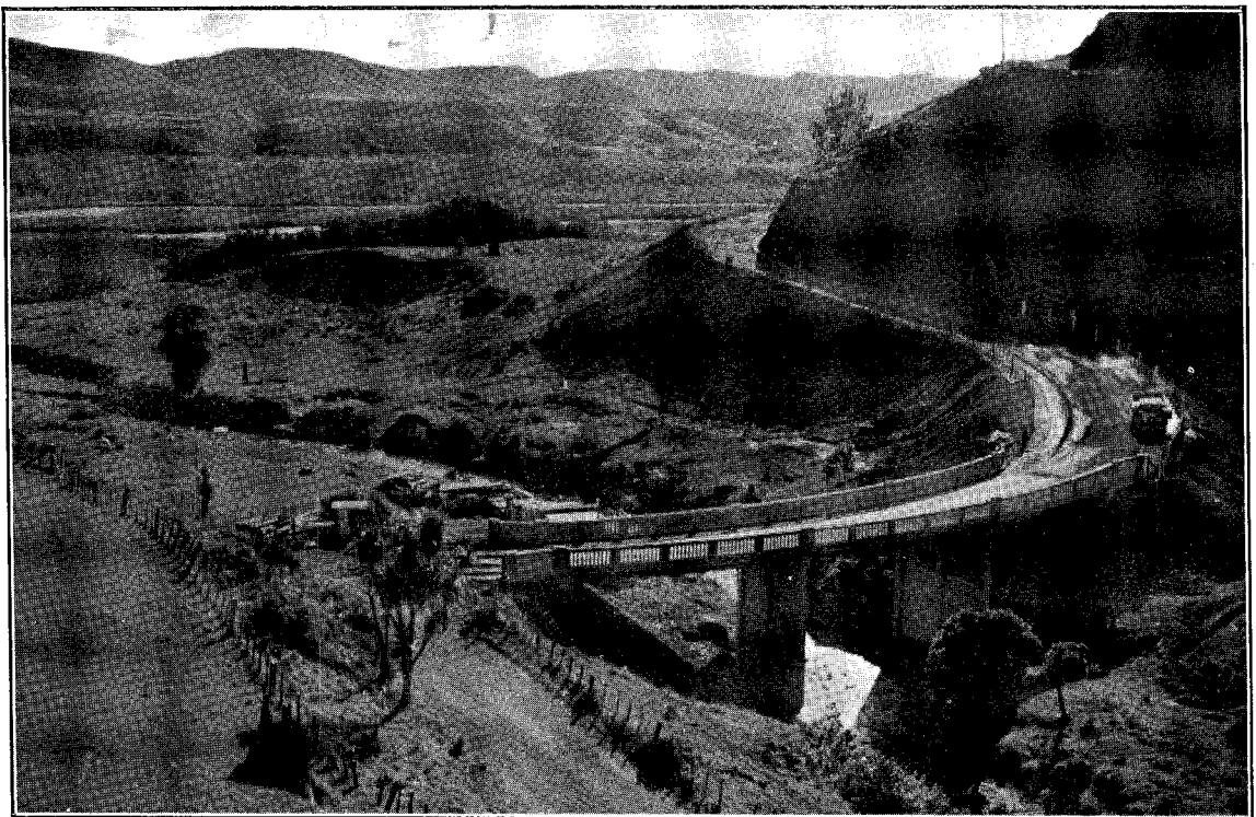
CHURCH HILL DEVIATION AND BRIDGE; THREE 40 FT. SPANS, 24 FT. ROADWAY. POHANGINA VALLEY MAIN HIGHWAY.
