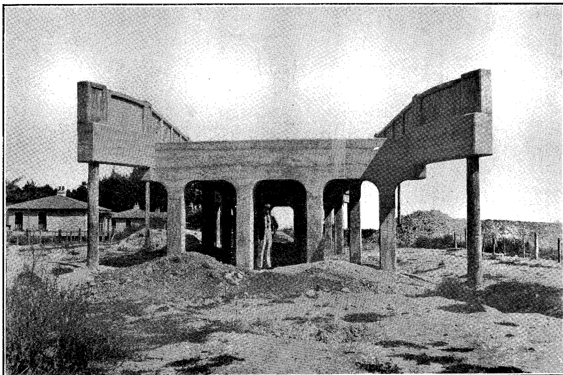
GREATFORD OVERBRIDGE UNDER CONSTRUCTION. END VIEW BEFORE PLACING APPROACH BANKS.
