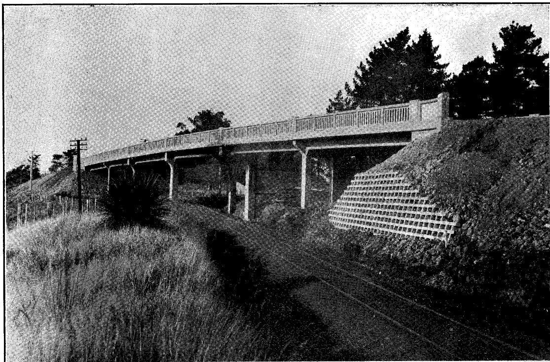
BONNY GLEN OVERBRIDGE. FOUR 40 FT., TWO 45 FT. SPANS, 24 FT. ROADWAY. BRIDGE SKEWED 72^{\circ} FROM NORMAL, NECESSITATING "STEPOVER" PIER. TURAKINA-CLIFF ROAD VIA MARTON MAIN HIGHWAY.
