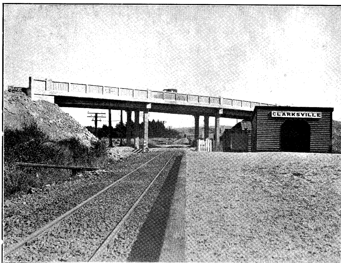
CLARKSVILLE OVERBRIDGE. THREE 45 FT. SPANS, 24 FT. ROADWAY, SKEWED 53^{\circ} FROM NORMAL.
