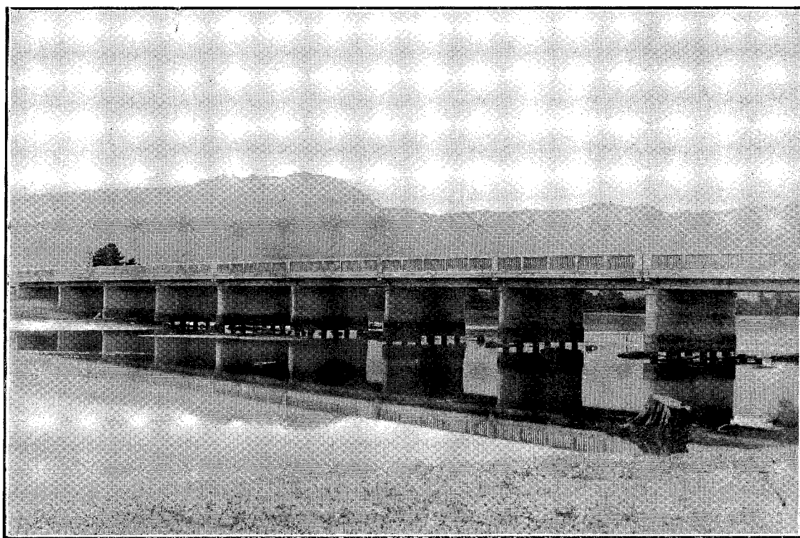
OROWAITI RIVER BRIDGE. TWELVE 40 FT. SPANS, 20 FT. ROADWAY, 4 FT. FOOTWAY. WESTPORT-KARAMEA MAIN HIGHWAY.
