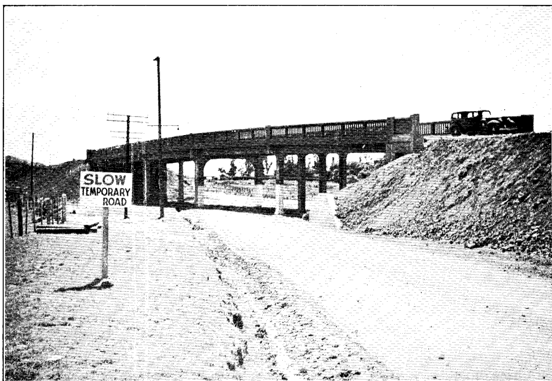
LEVEL-CROSSING ELIMINATION, OVERBRIDGE, 10 M. 49 CH. RAILWAY FORMATION IN USE AS TEMPORARY ROAD.
